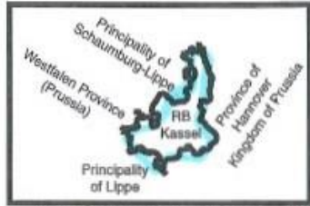
Discontinuous region located about 45 miles northwest of the main district
