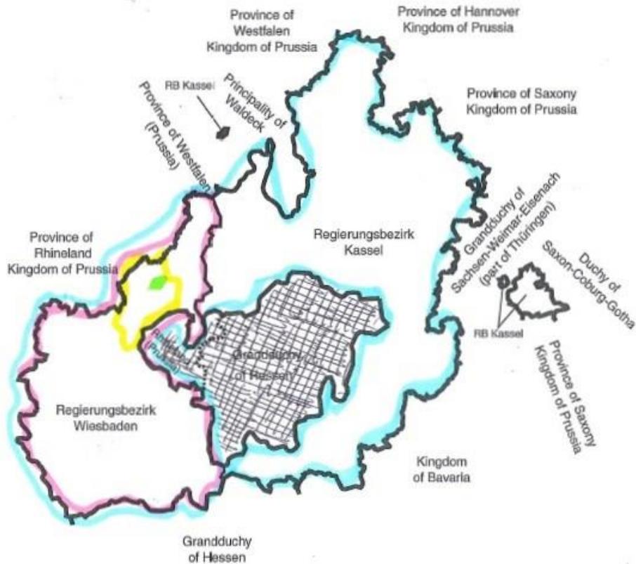
Discontinuous region located about 45 miles northwest of the main district
